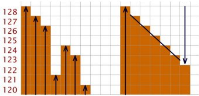
Lossy method
