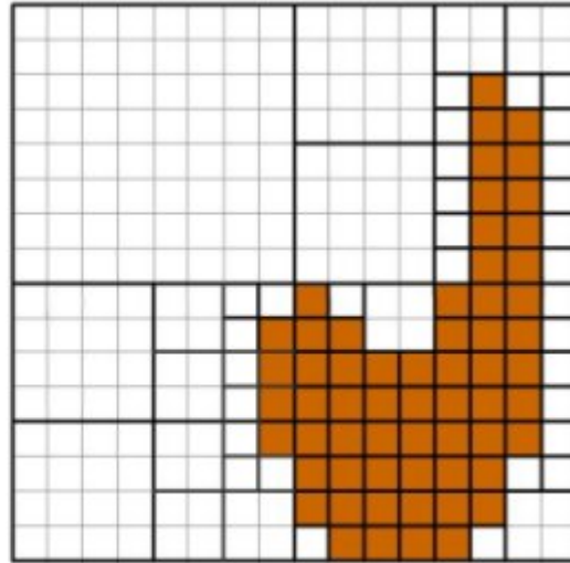
Quadtree representation
